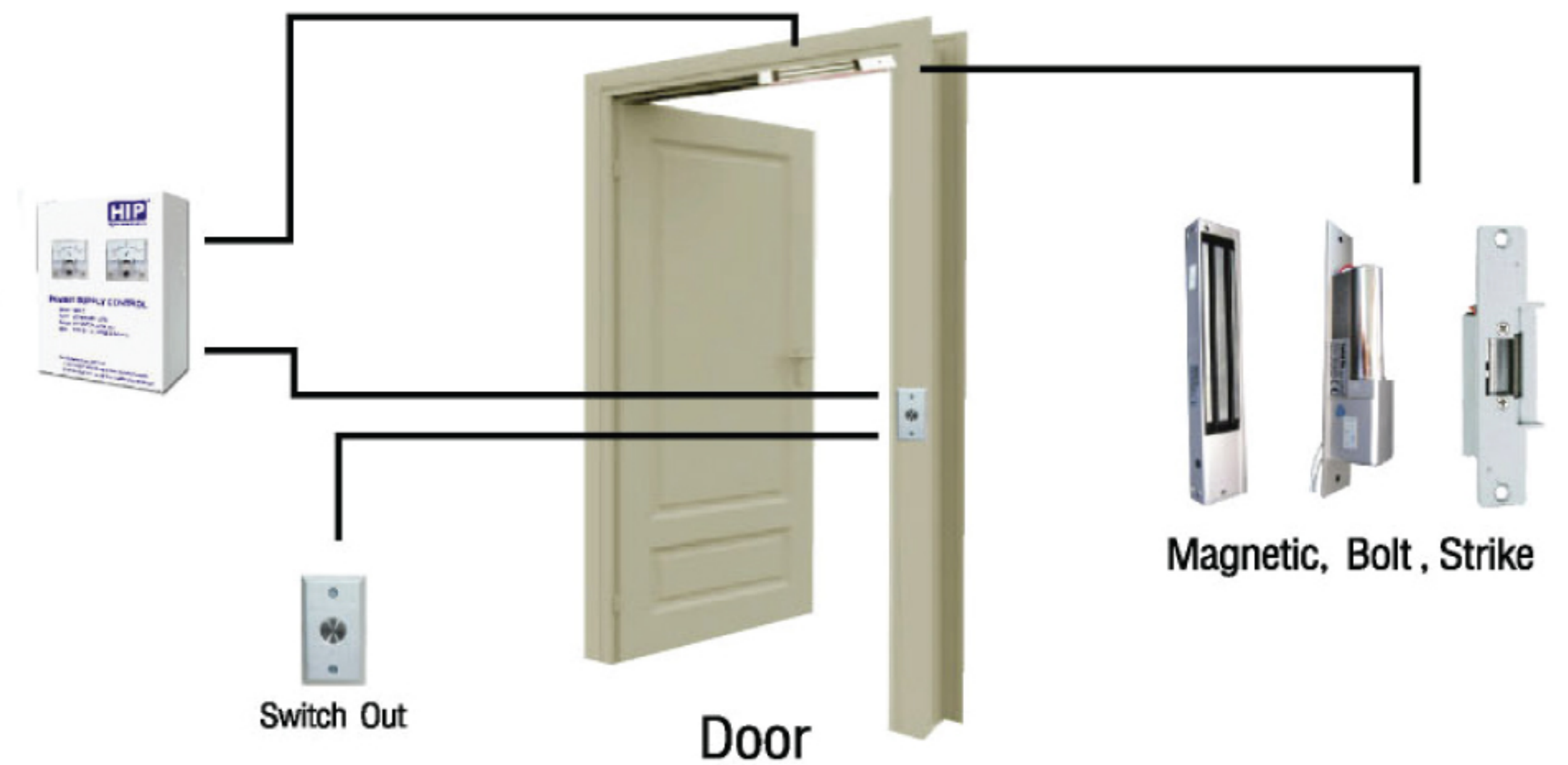
Connection Type Access Control System
